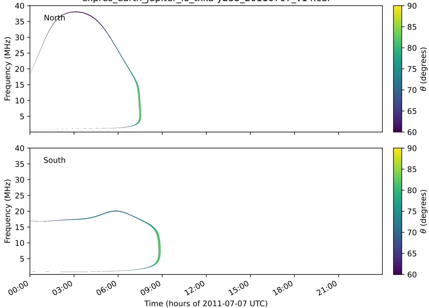
expres_earth_jupiter_io_txka-y235_20110707_v14.cdf
