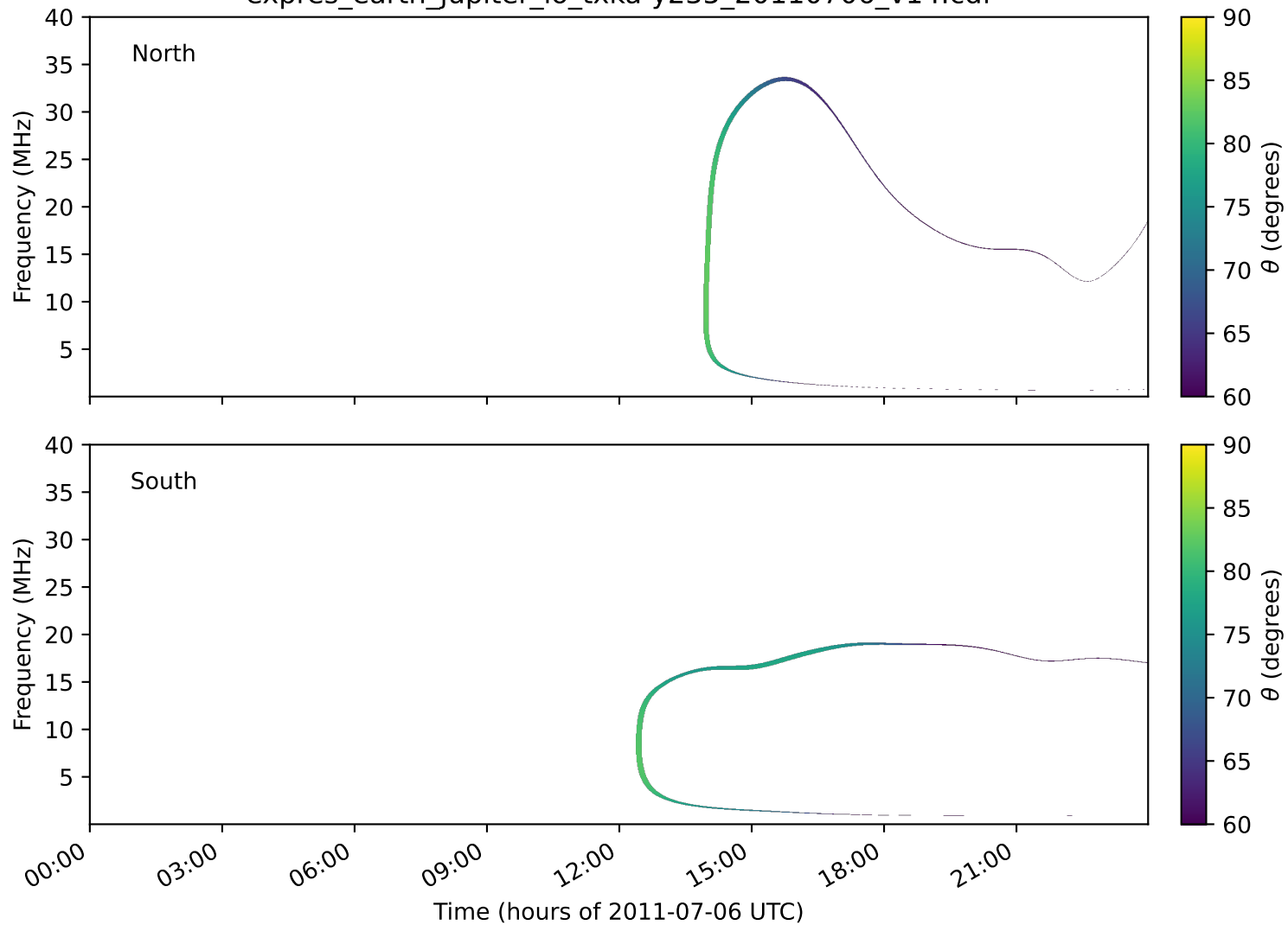
expres_earth_jupiter_io_txka-y235_20110706_v14.cdf
