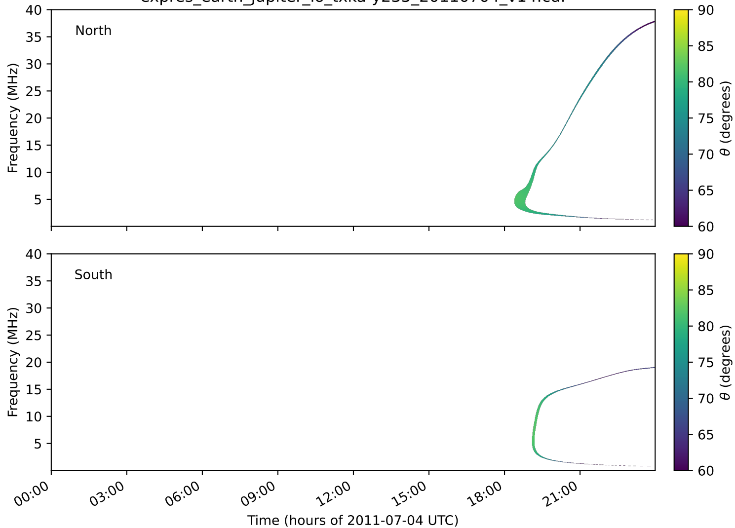
expres_earth_jupiter_io_txka-y235_20110704_v14.cdf
