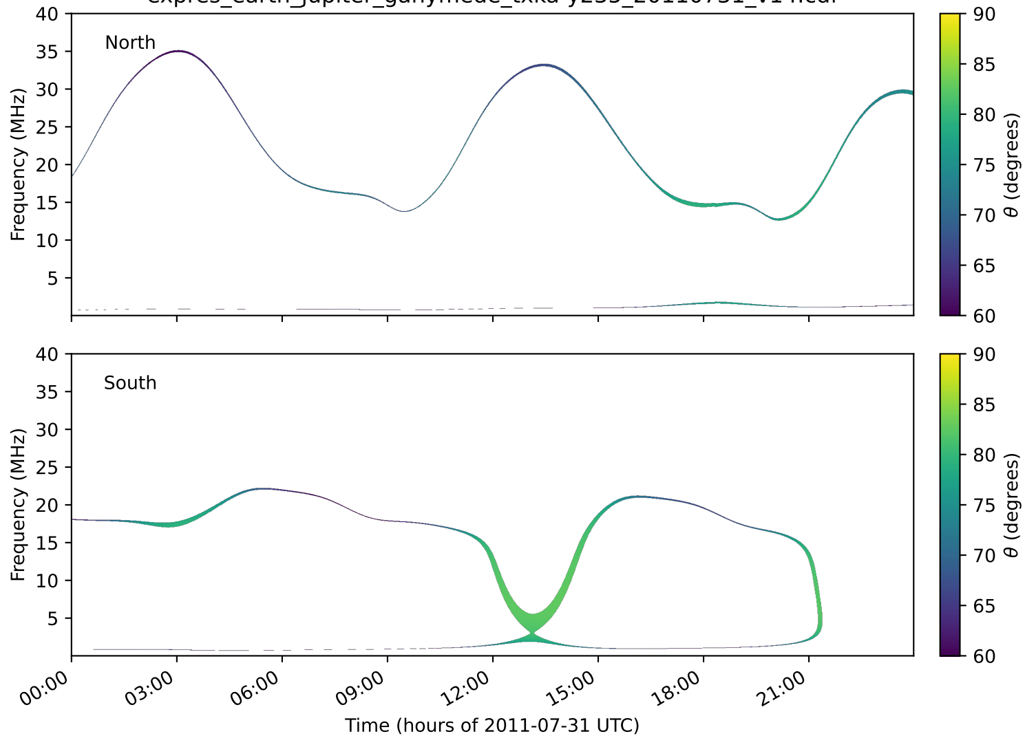
expres_earth_jupiter_ganymede_txka-y235_20110731_v14.cdf
