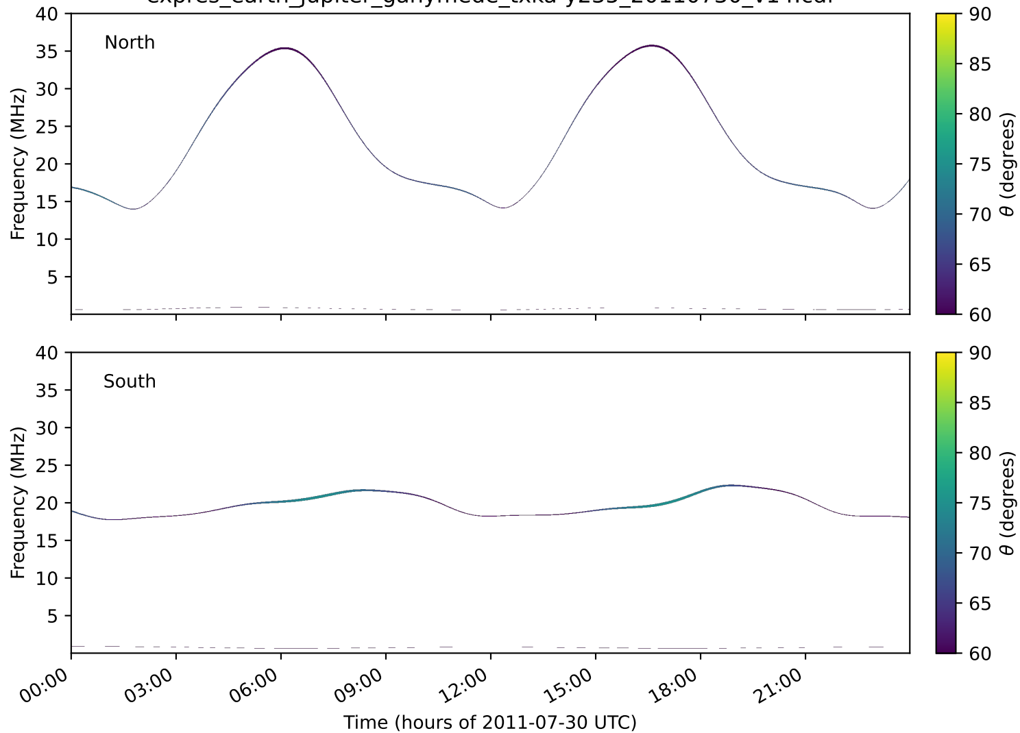
expres_earth_jupiter_ganymede_txka-y235_20110730_v14.cdf
