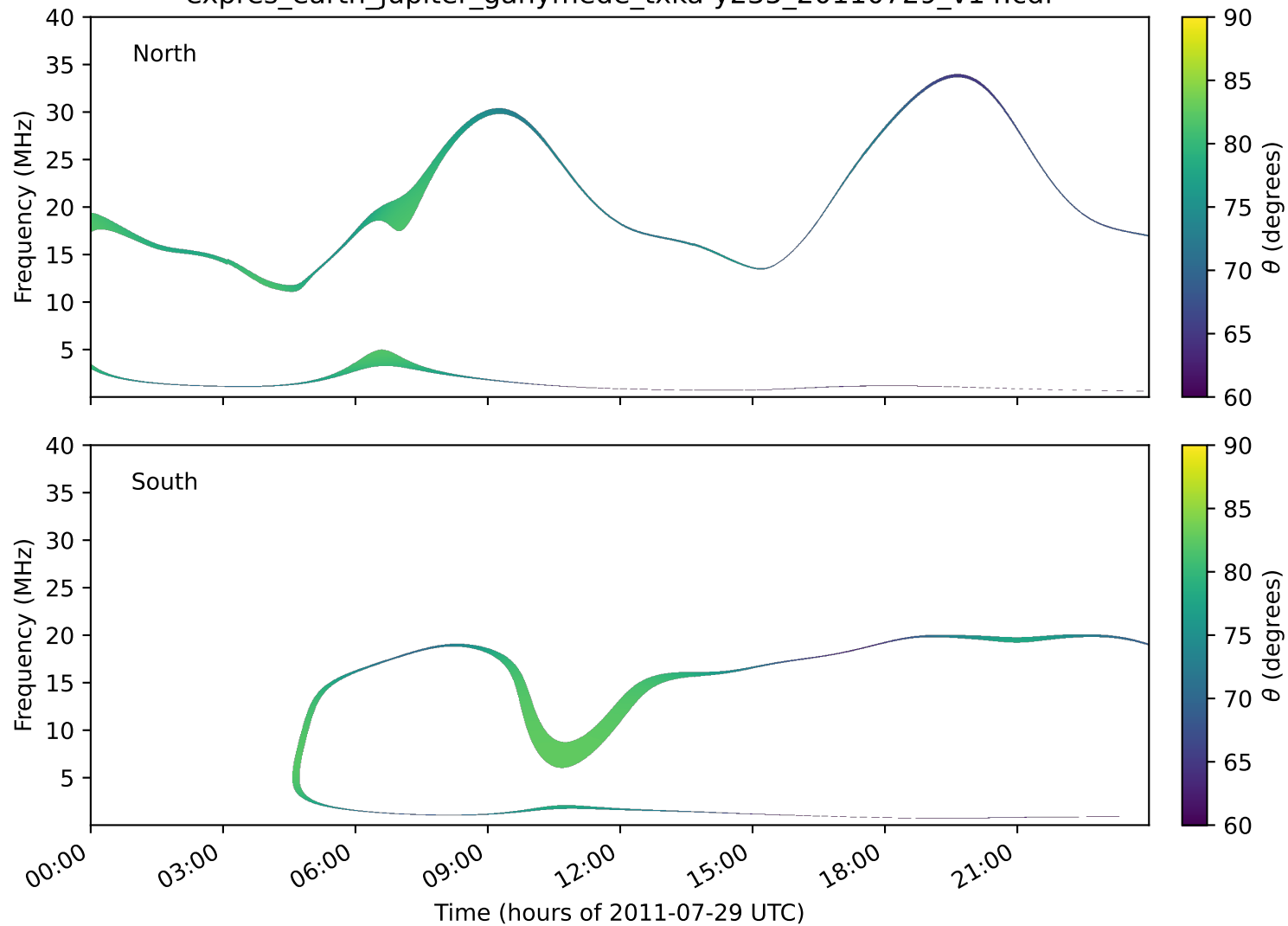
expres_earth_jupiter_ganymede_txka-y235_20110729_v14.cdf
