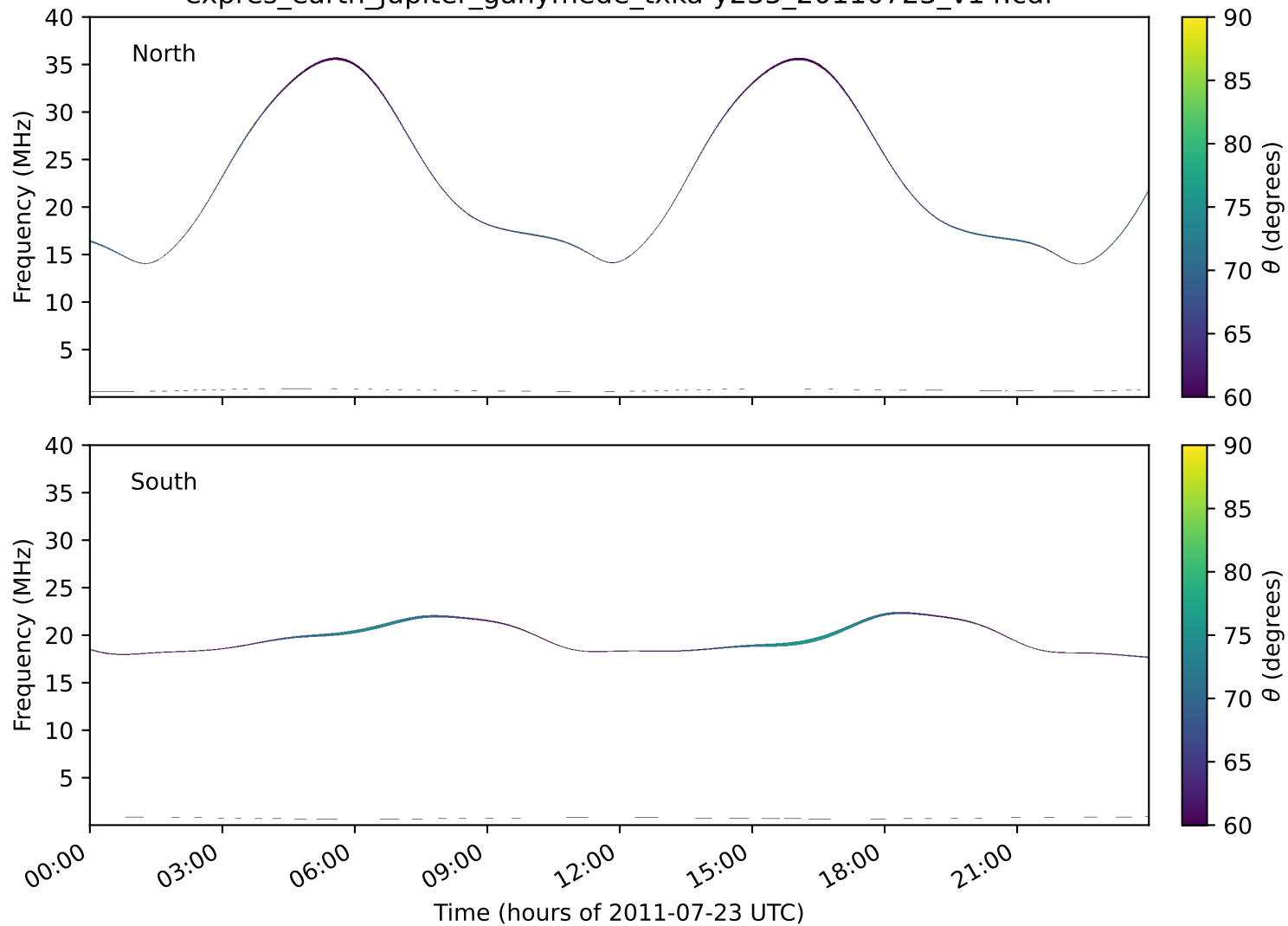
expres_earth_jupiter_ganymede_txka-y235_20110723_v14.cdf
