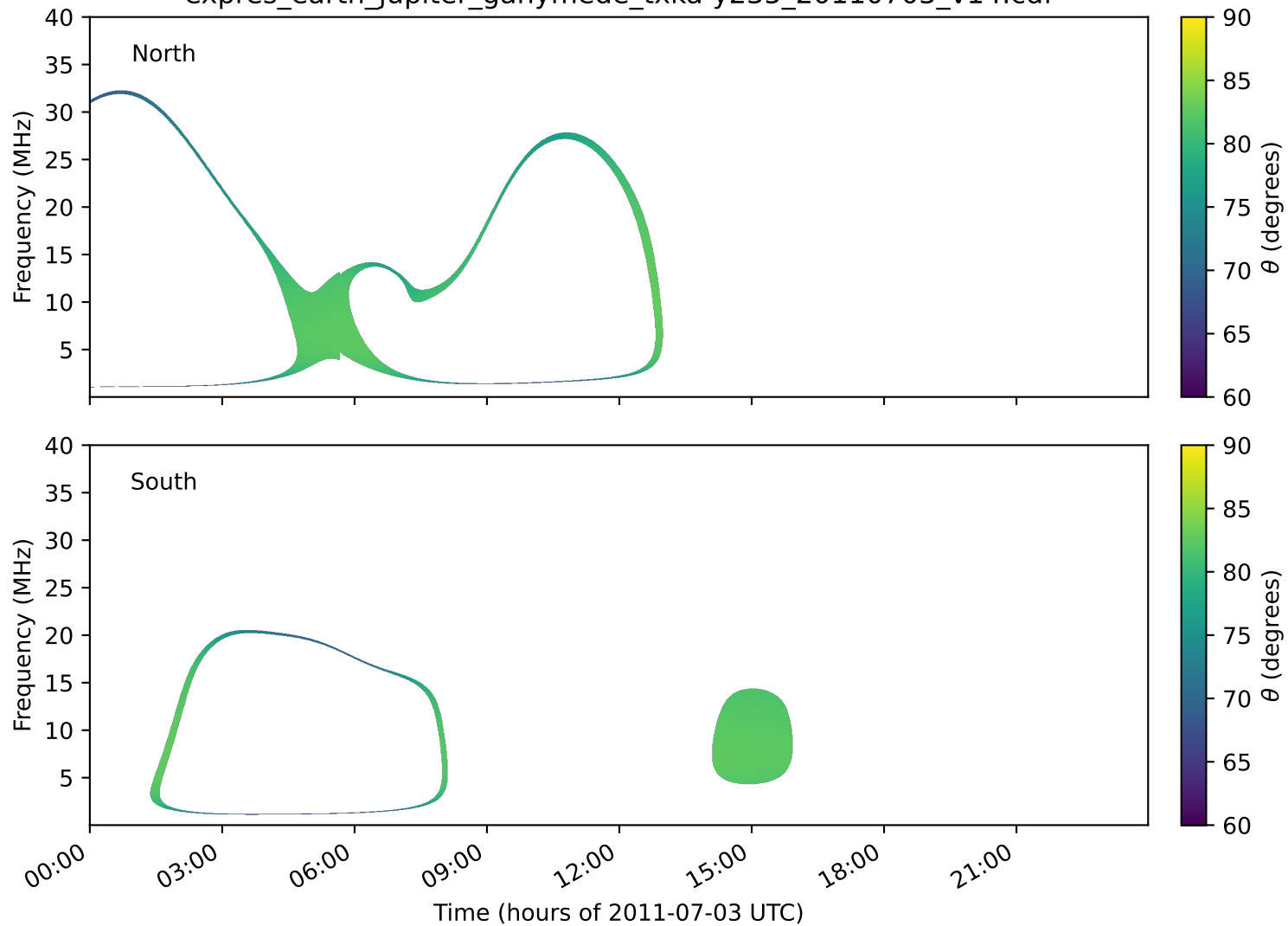
expres_earth_jupiter_ganymede_txka-y235_20110703_v14.cdf
