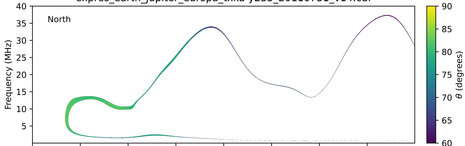
expres_earth_jupiter_europa_txka-y235_20110731_v14.cdf
