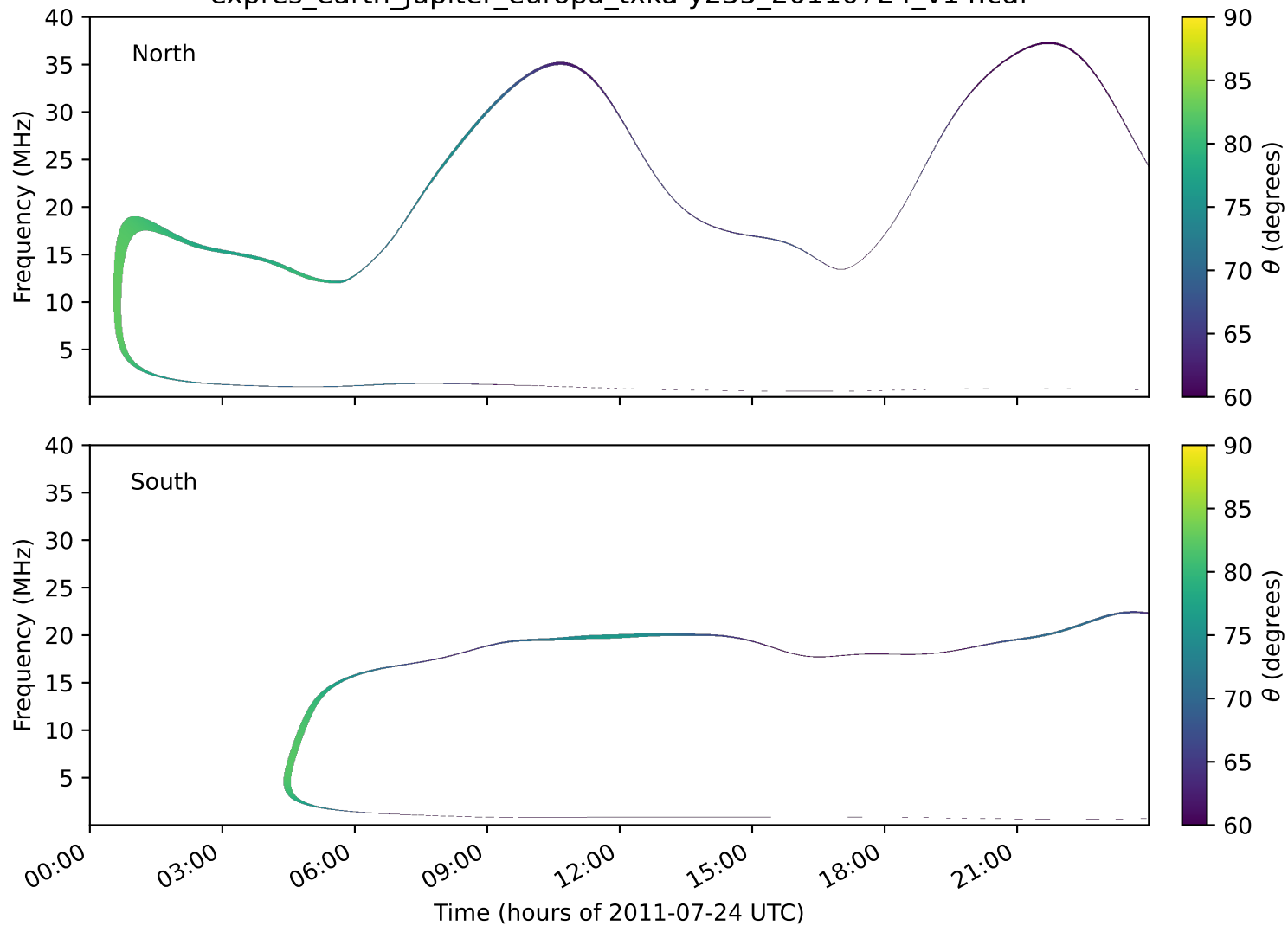
expres_earth_jupiter_europa_txka-y235_20110724_v14.cdf
