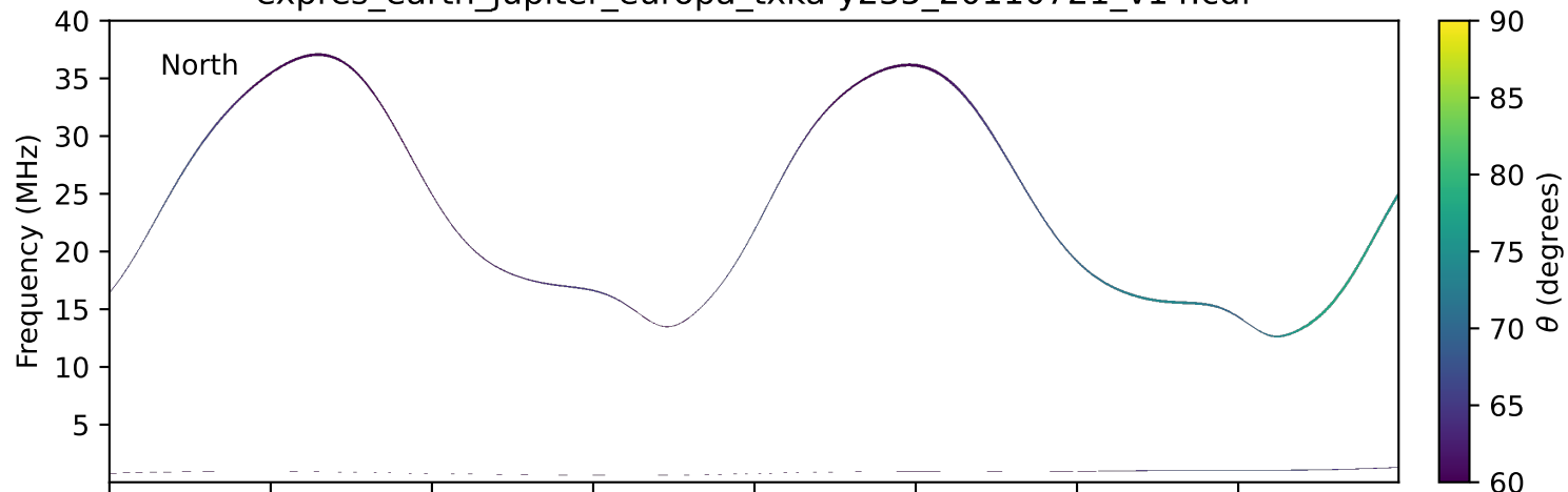
expres_earth_jupiter_europa_txka-y235_20110721_v14.cdf
