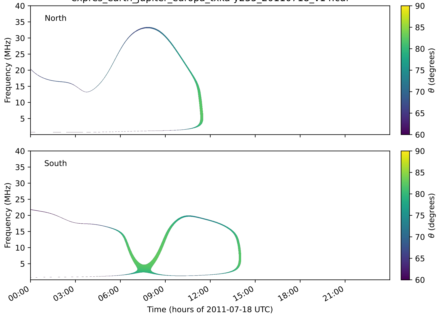
expres_earth_jupiter_europa_txka-y235_20110718_v14.cdf
