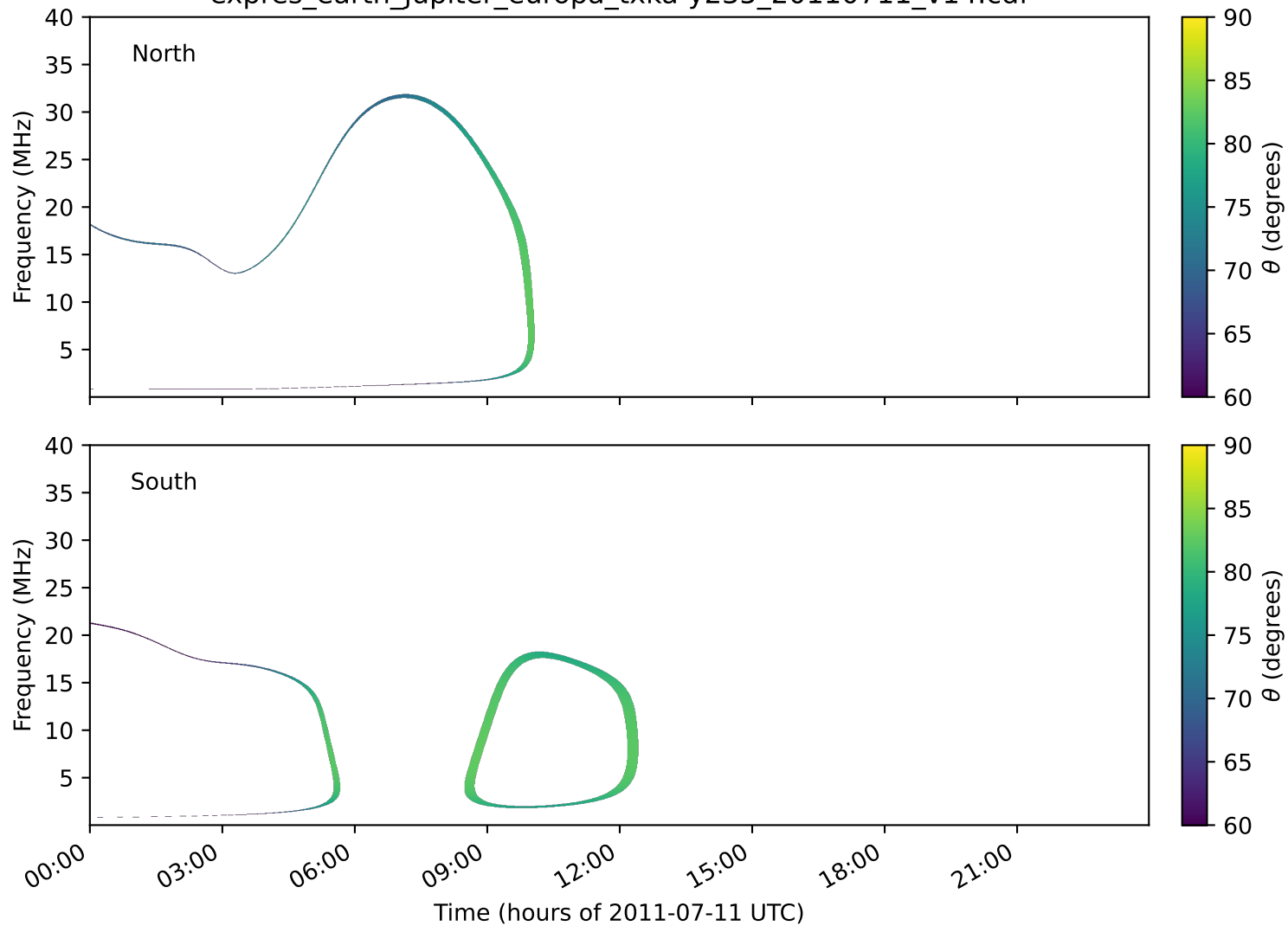
expres_earth_jupiter_europa_txka-y235_20110711_v14.cdf
