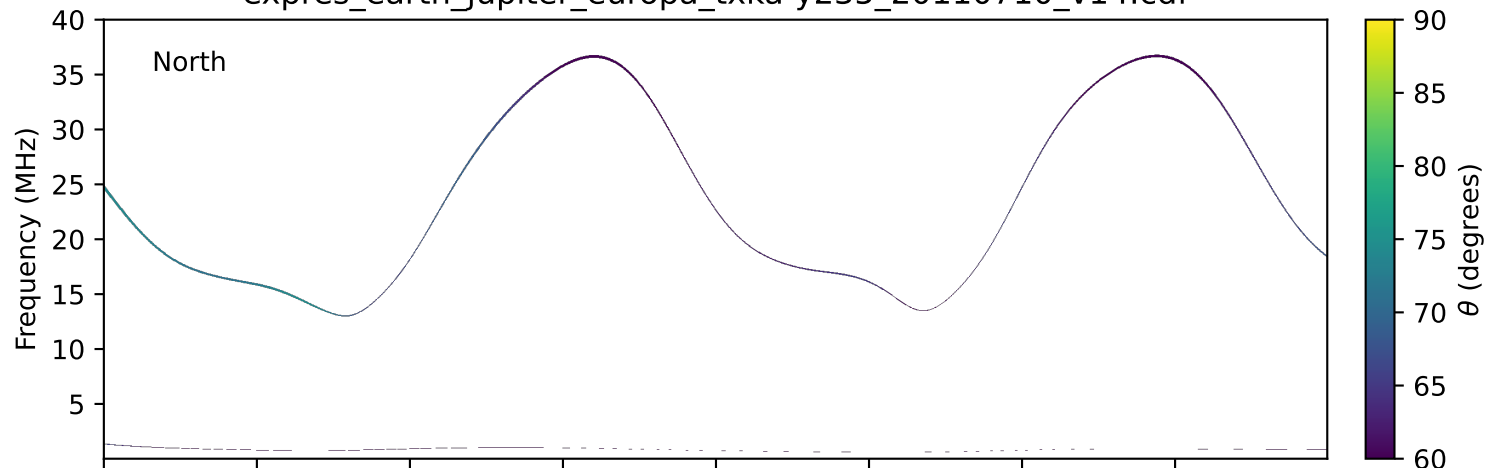
expres_earth_jupiter_europa_txka-y235_20110710_v14.cdf
