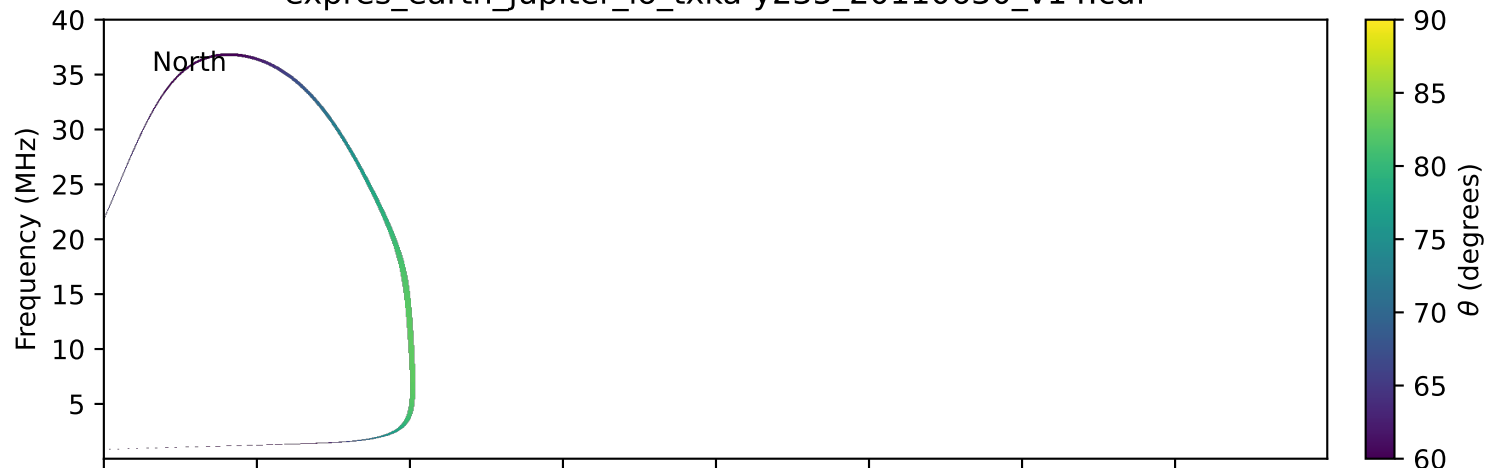
expres_earth_jupiter_io_txka-y235_20110630_v14.cdf
