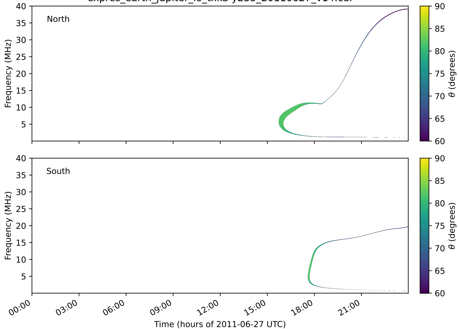
expres_earth_jupiter_io_txka-y235_20110627_v14.cdf
