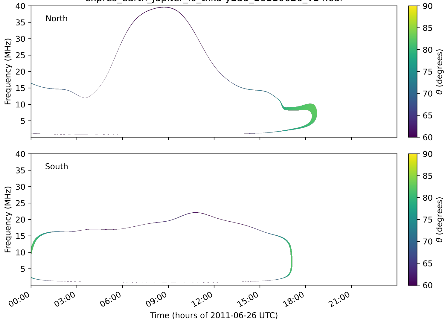
expres_earth_jupiter_io_txka-y235_20110626_v14.cdf
