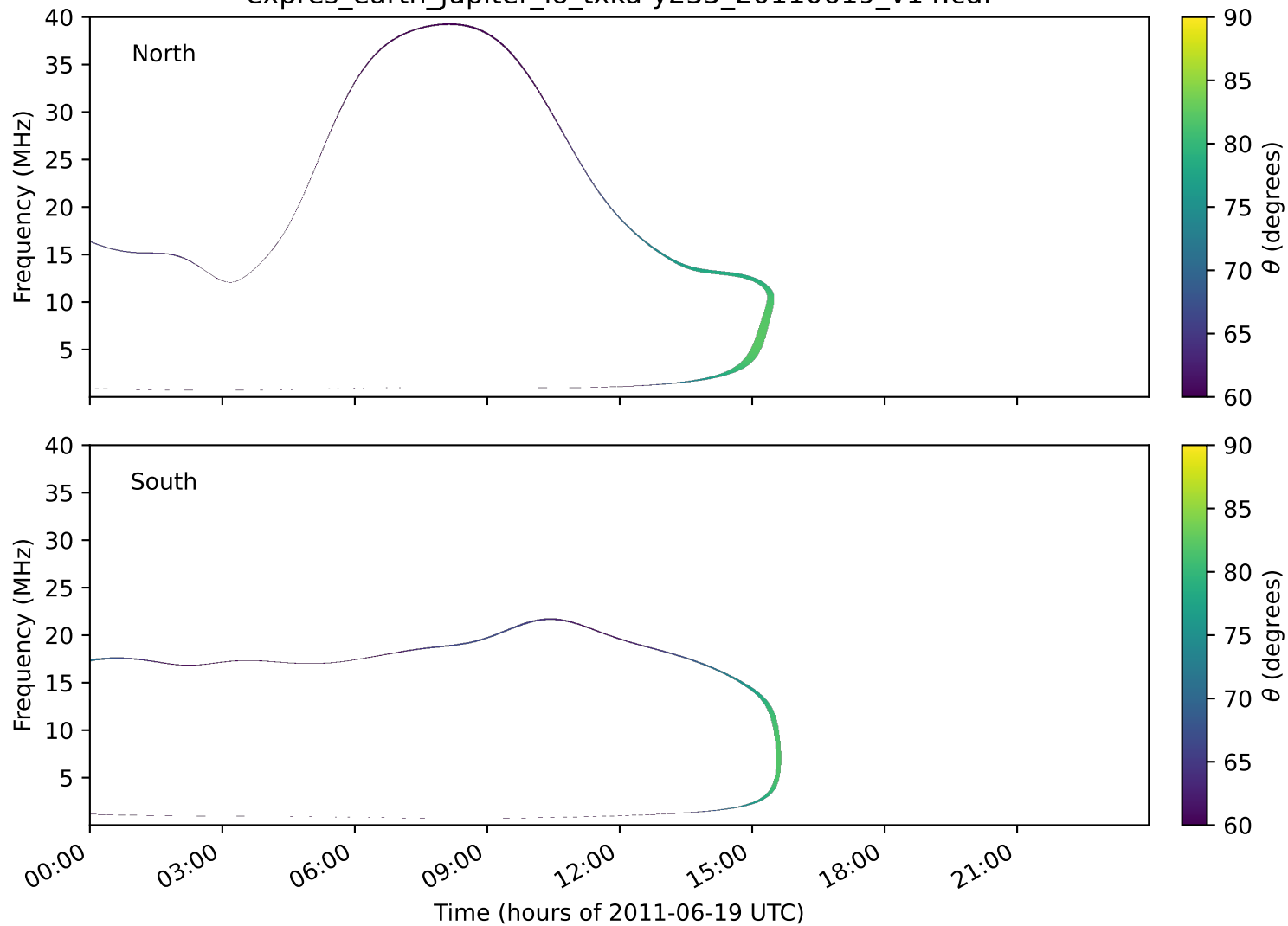
expres_earth_jupiter_io_txka-y235_20110619_v14.cdf
