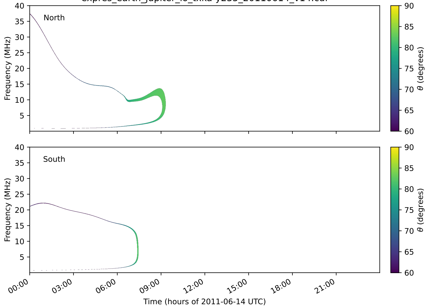
expres_earth_jupiter_io_txka-y235_20110614_v14.cdf
