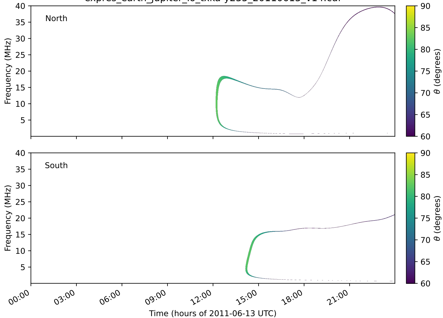
expres_earth_jupiter_io_txka-y235_20110613_v14.cdf
