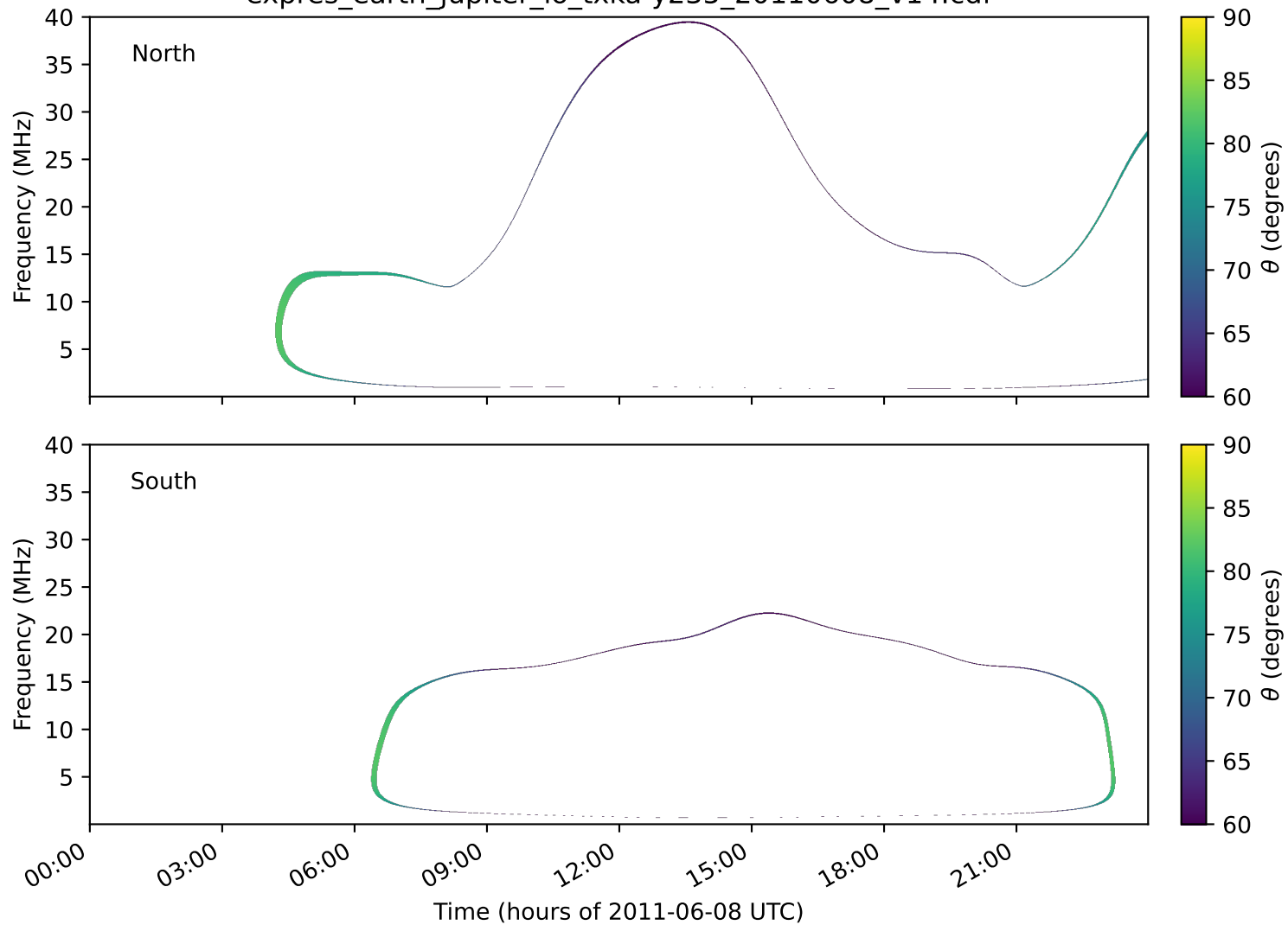
expres_earth_jupiter_io_txka-y235_20110608_v14.cdf
