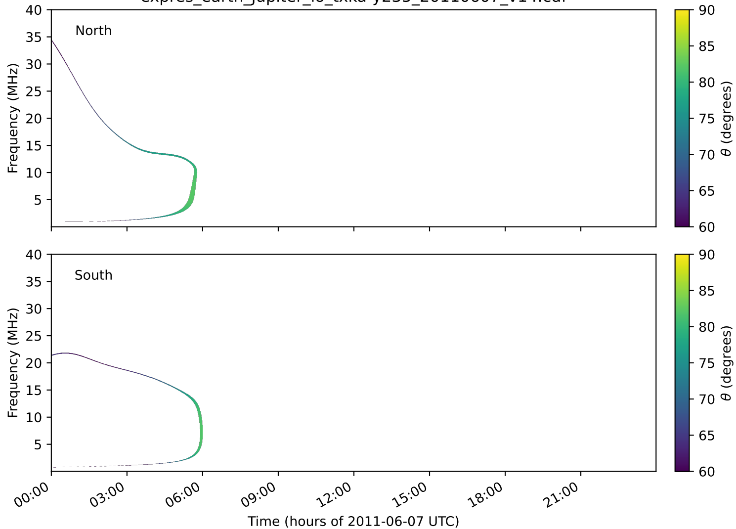
expres_earth_jupiter_io_txka-y235_20110607_v14.cdf
