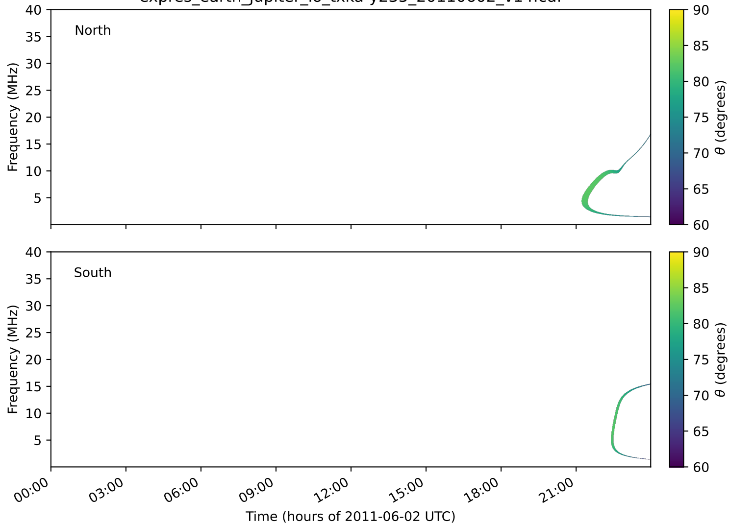
expres_earth_jupiter_io_txka-y235_20110602_v14.cdf
