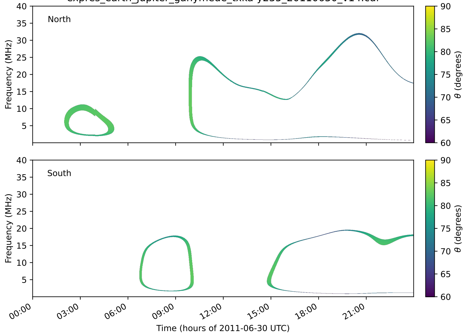
expres_earth_jupiter_ganymede_txka-y235_20110630_v14.cdf
