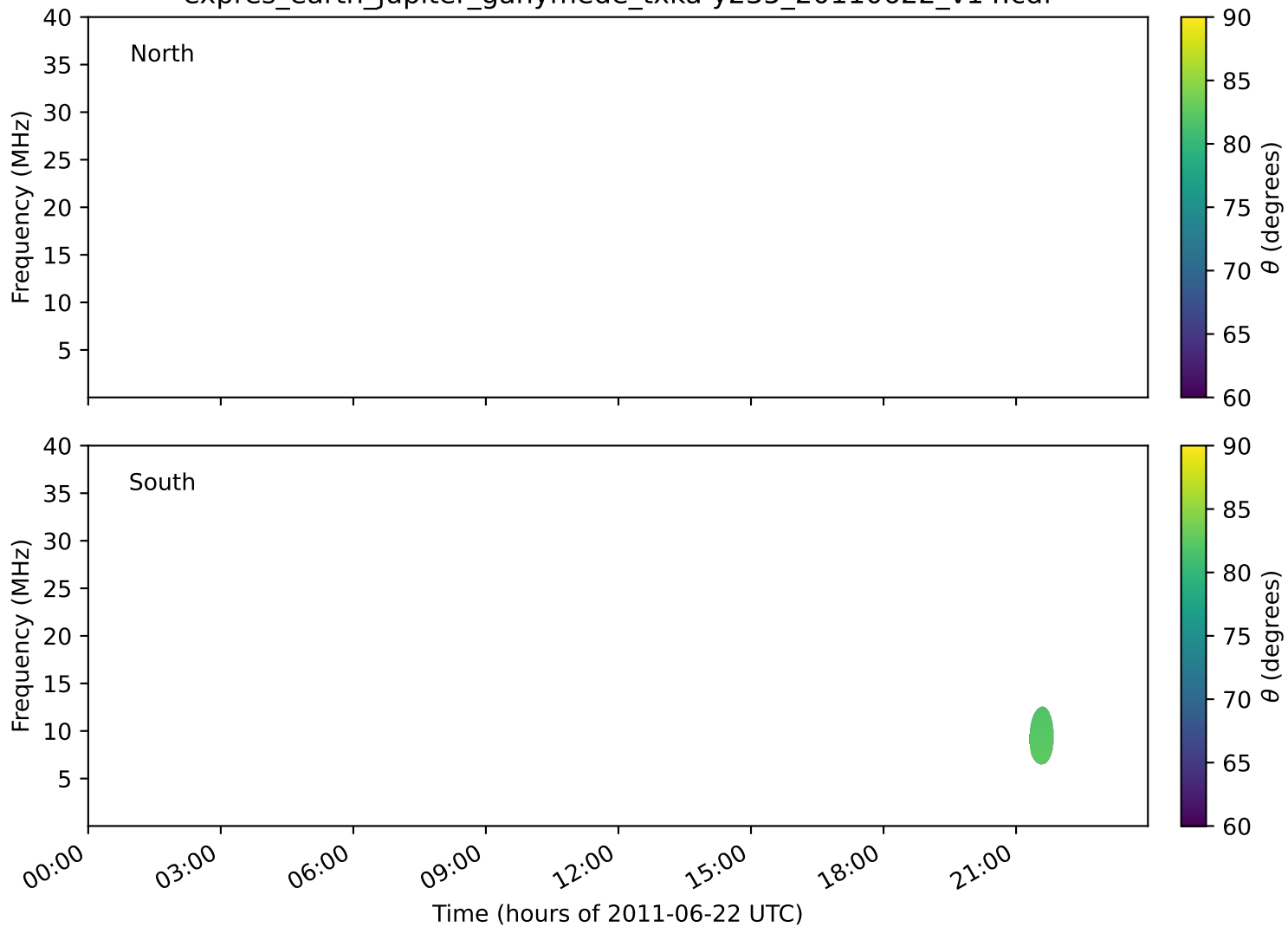
expres_earth_jupiter_ganymede_txka-y235_20110622_v14.cdf
