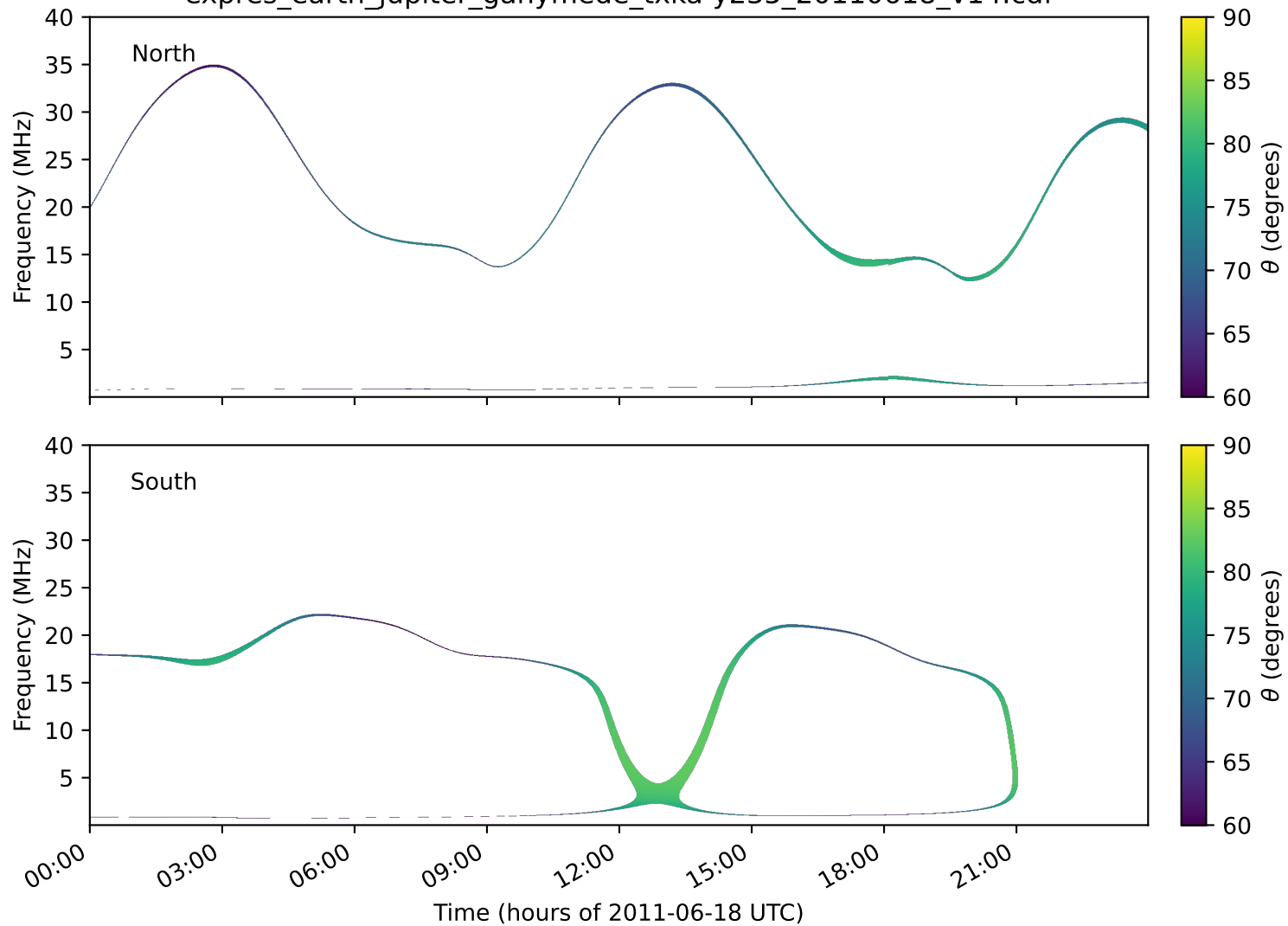
expres_earth_jupiter_ganymede_txka-y235_20110618_v14.cdf
