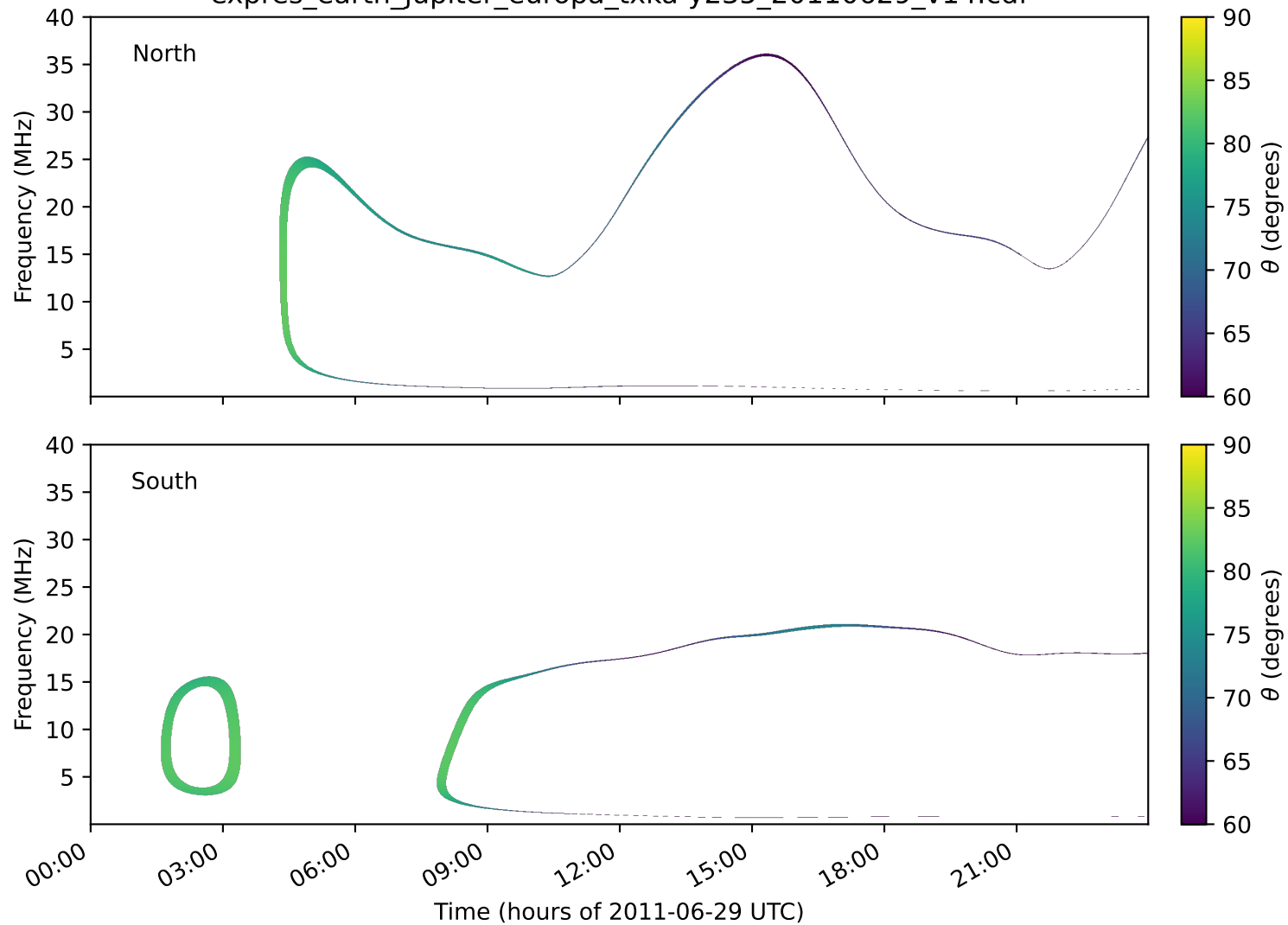
expres_earth_jupiter_europa_txka-y235_20110629_v14.cdf
