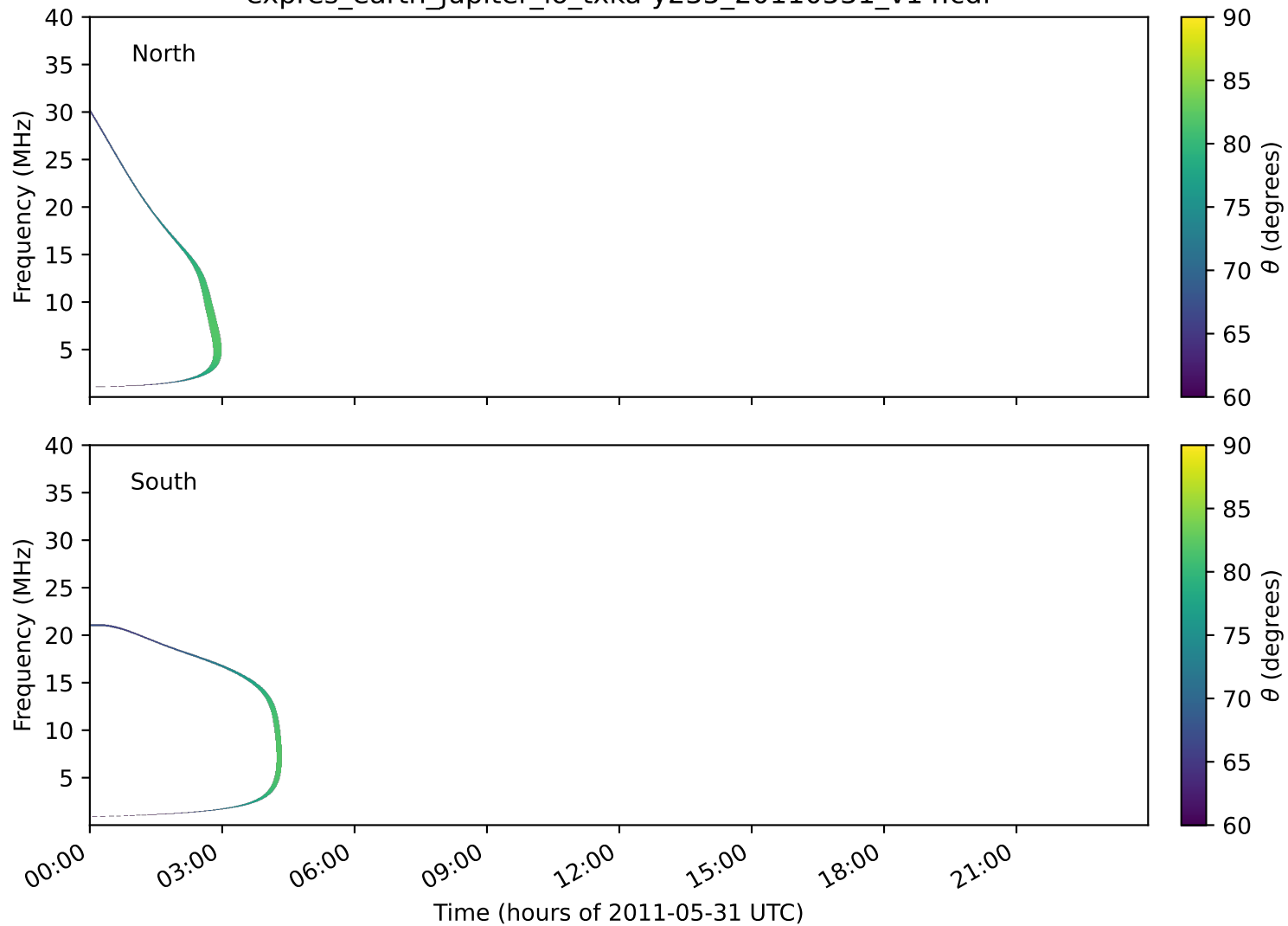
expres_earth_jupiter_io_txka-y235_20110531_v14.cdf
