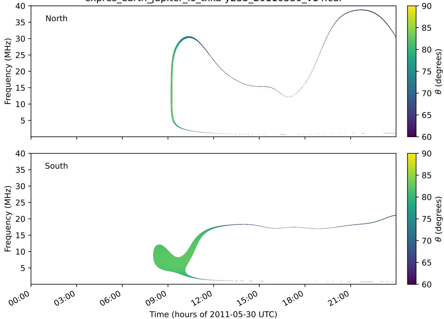
expres_earth_jupiter_io_txka-y235_20110530_v14.cdf
