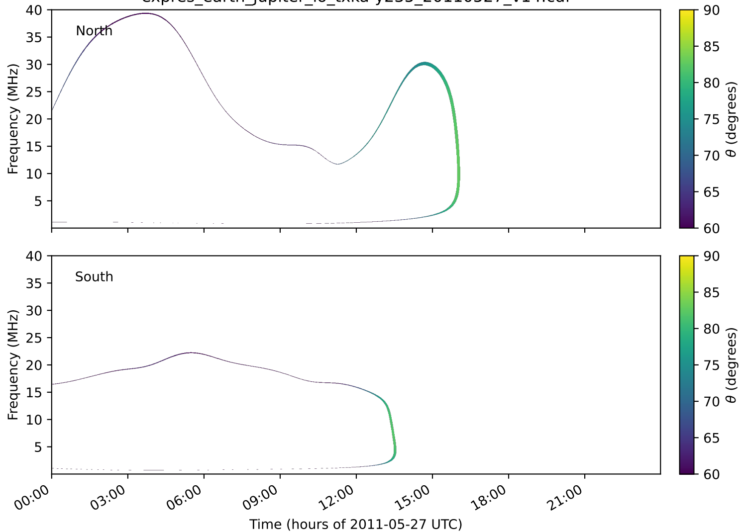
expres_earth_jupiter_io_txka-y235_20110527_v14.cdf
