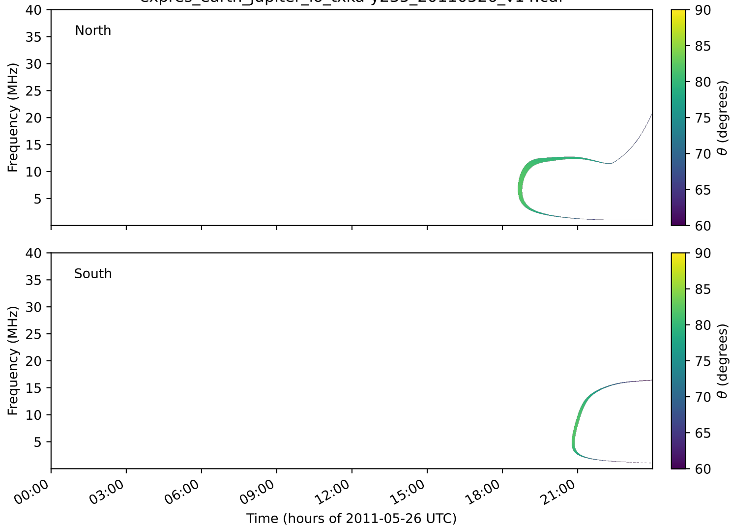
expres_earth_jupiter_io_txka-y235_20110526_v14.cdf
