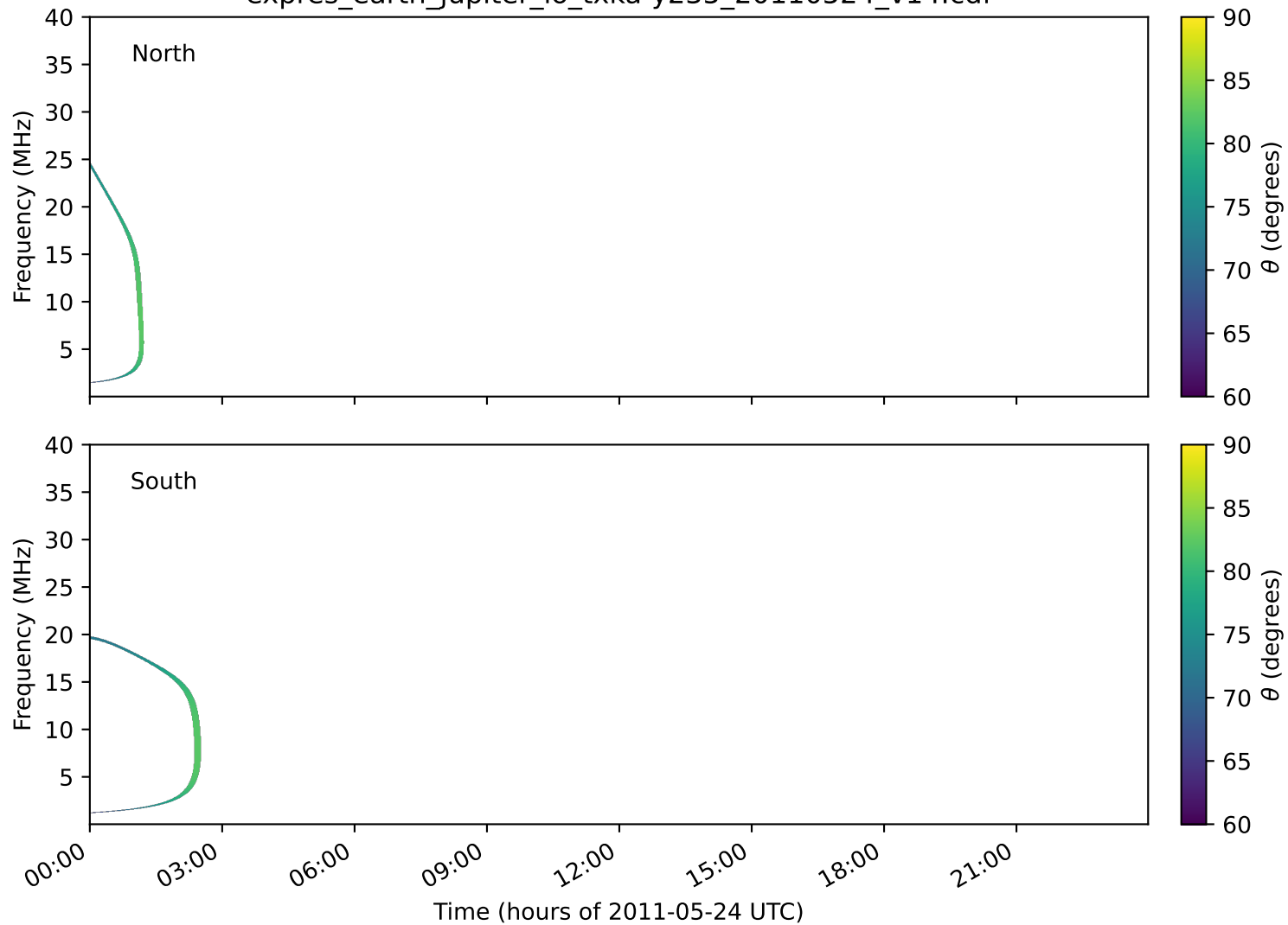
expres_earth_jupiter_io_txka-y235_20110524_v14.cdf
