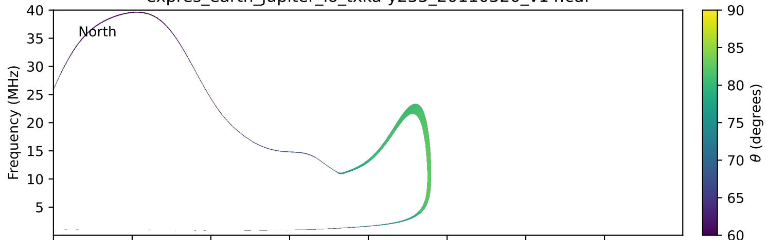
expres_earth_jupiter_io_txka-y235_20110520_v14.cdf
