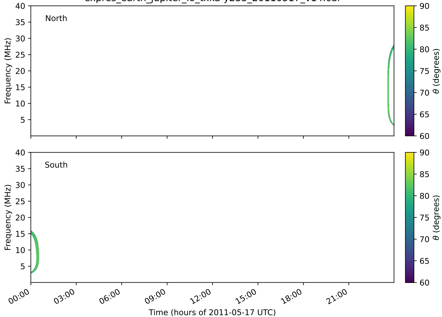
expres_earth_jupiter_io_txka-y235_20110517_v14.cdf
