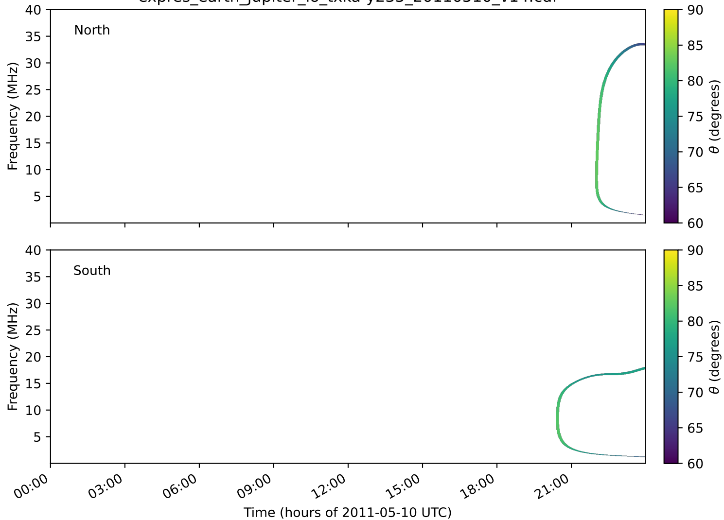
expres_earth_jupiter_io_txka-y235_20110510_v14.cdf
