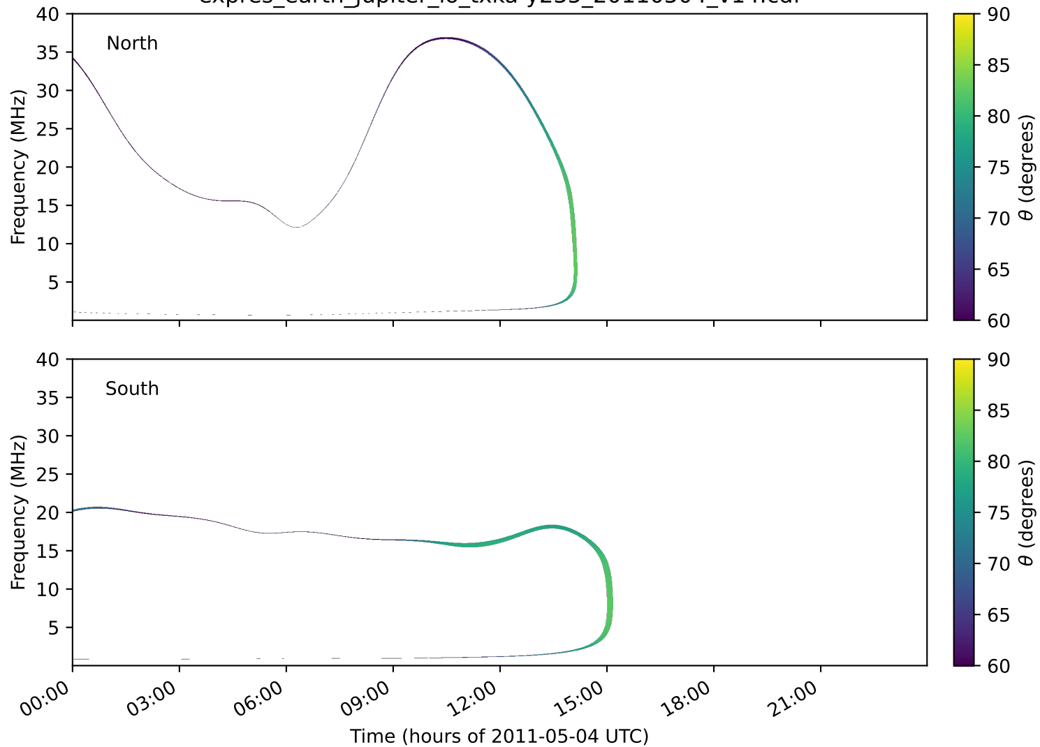
expres_earth_jupiter_io_txka-y235_20110504_v14.cdf
