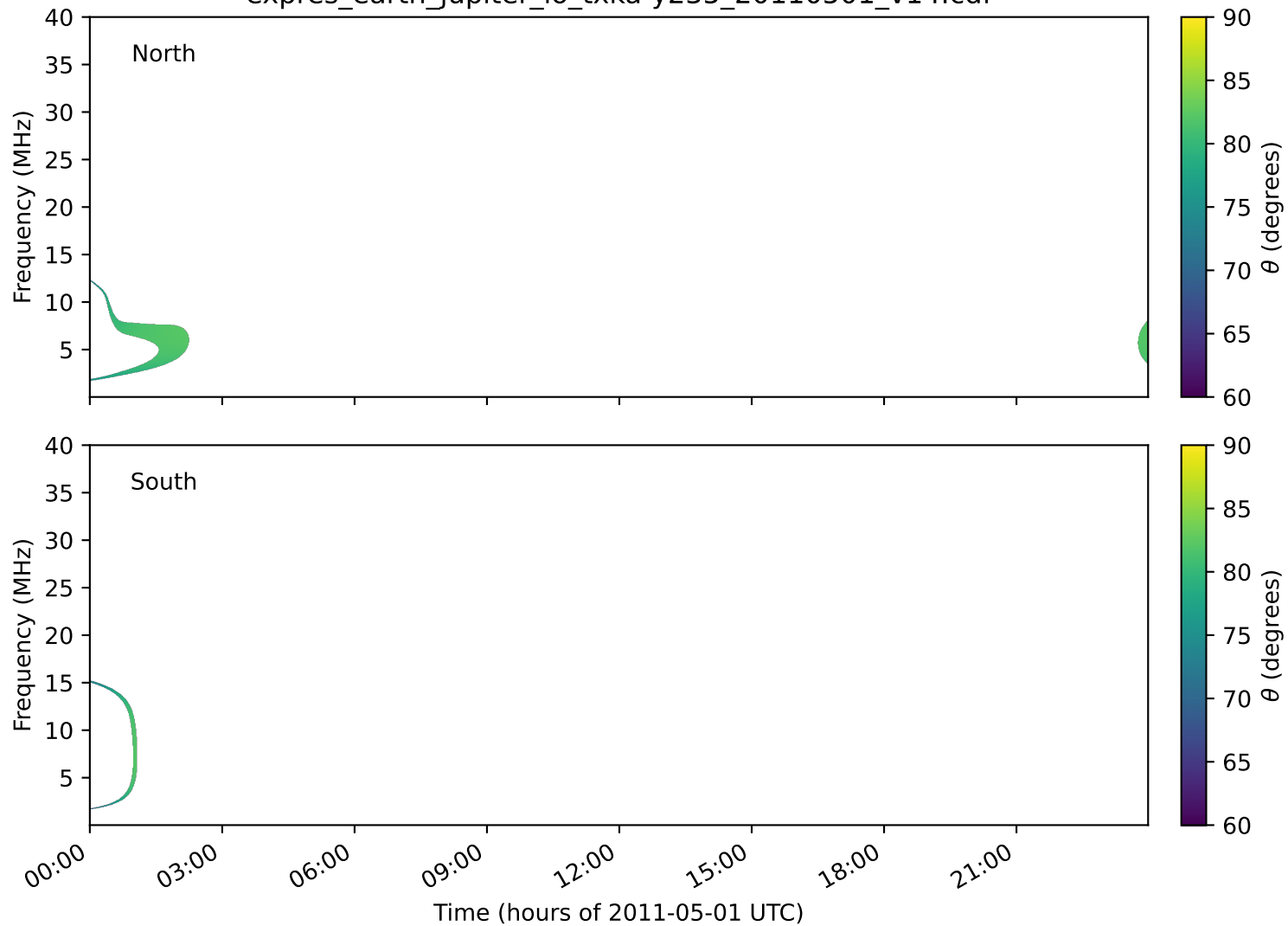
expres_earth_jupiter_io_txka-y235_20110501_v14.cdf
