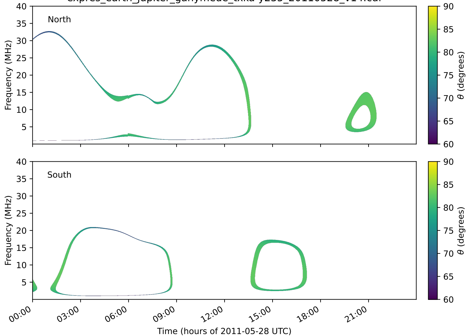
expres_earth_jupiter_ganymede_txka-y235_20110528_v14.cdf
