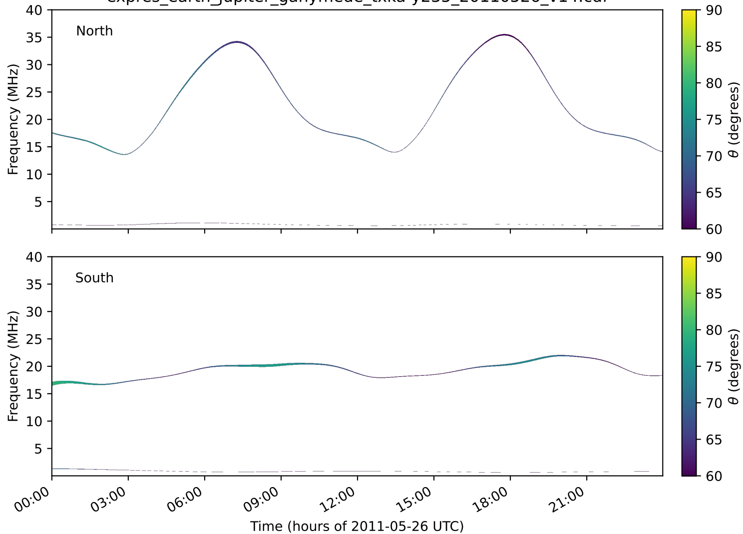
expres_earth_jupiter_ganymede_txka-y235_20110526_v14.cdf
