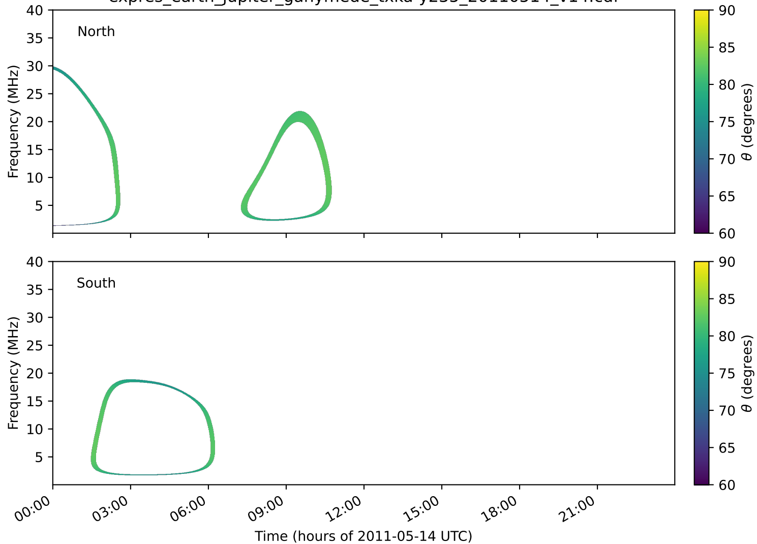
expres_earth_jupiter_ganymede_txka-y235_20110514_v14.cdf
