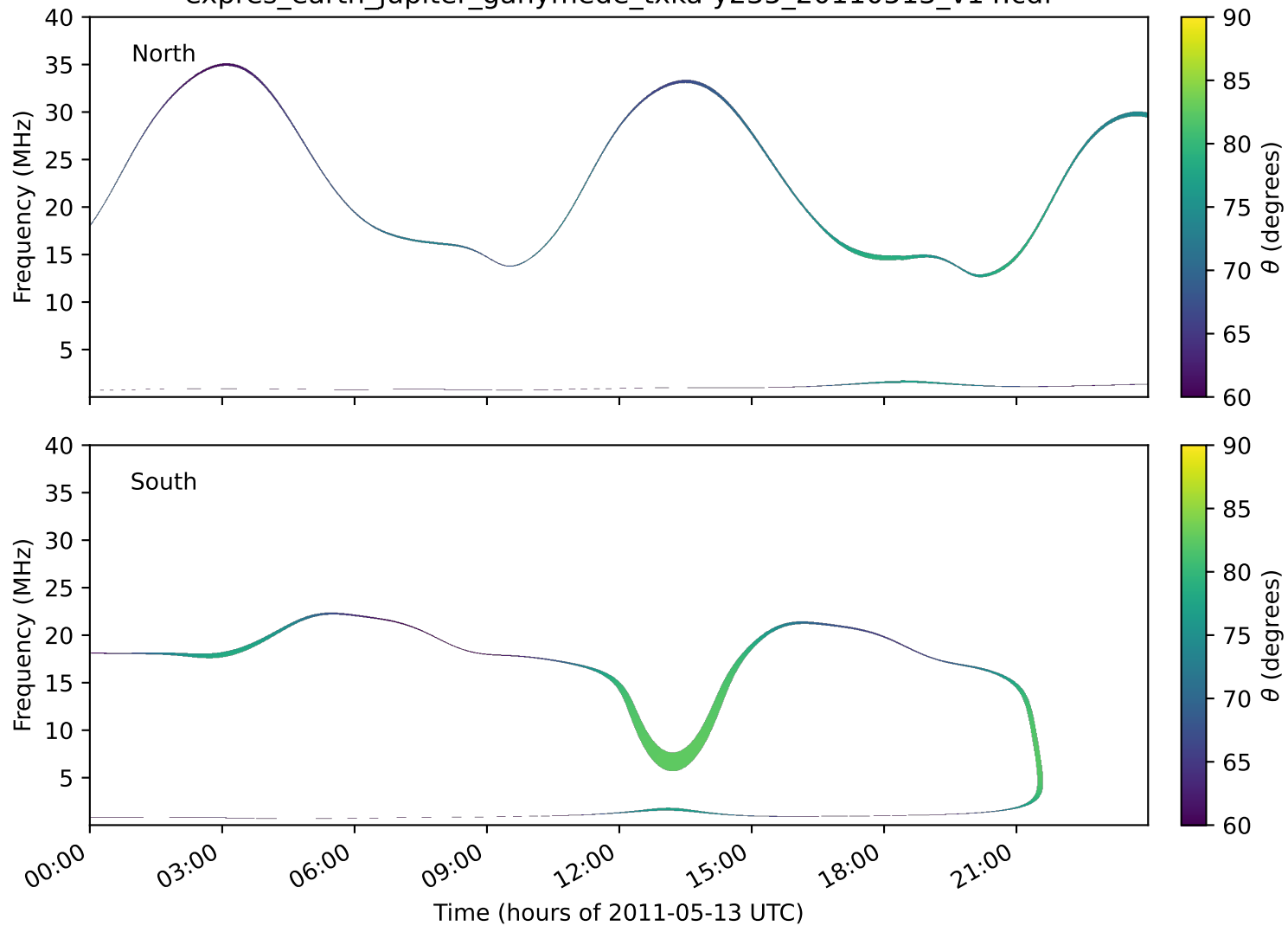
expres_earth_jupiter_ganymede_txka-y235_20110513_v14.cdf
