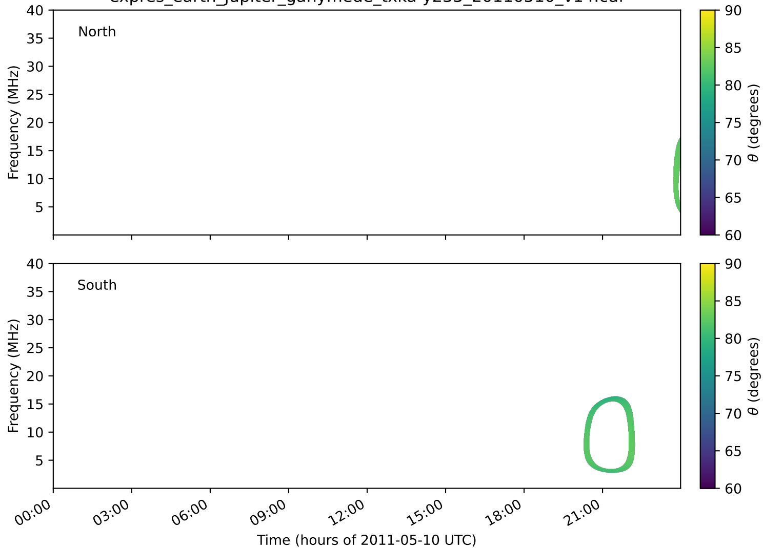
expres_earth_jupiter_ganymede_txka-y235_20110510_v14.cdf
