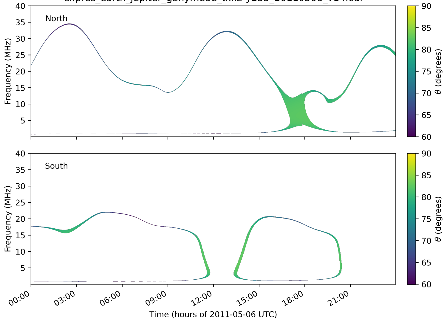
expres_earth_jupiter_ganymede_txka-y235_20110506_v14.cdf
