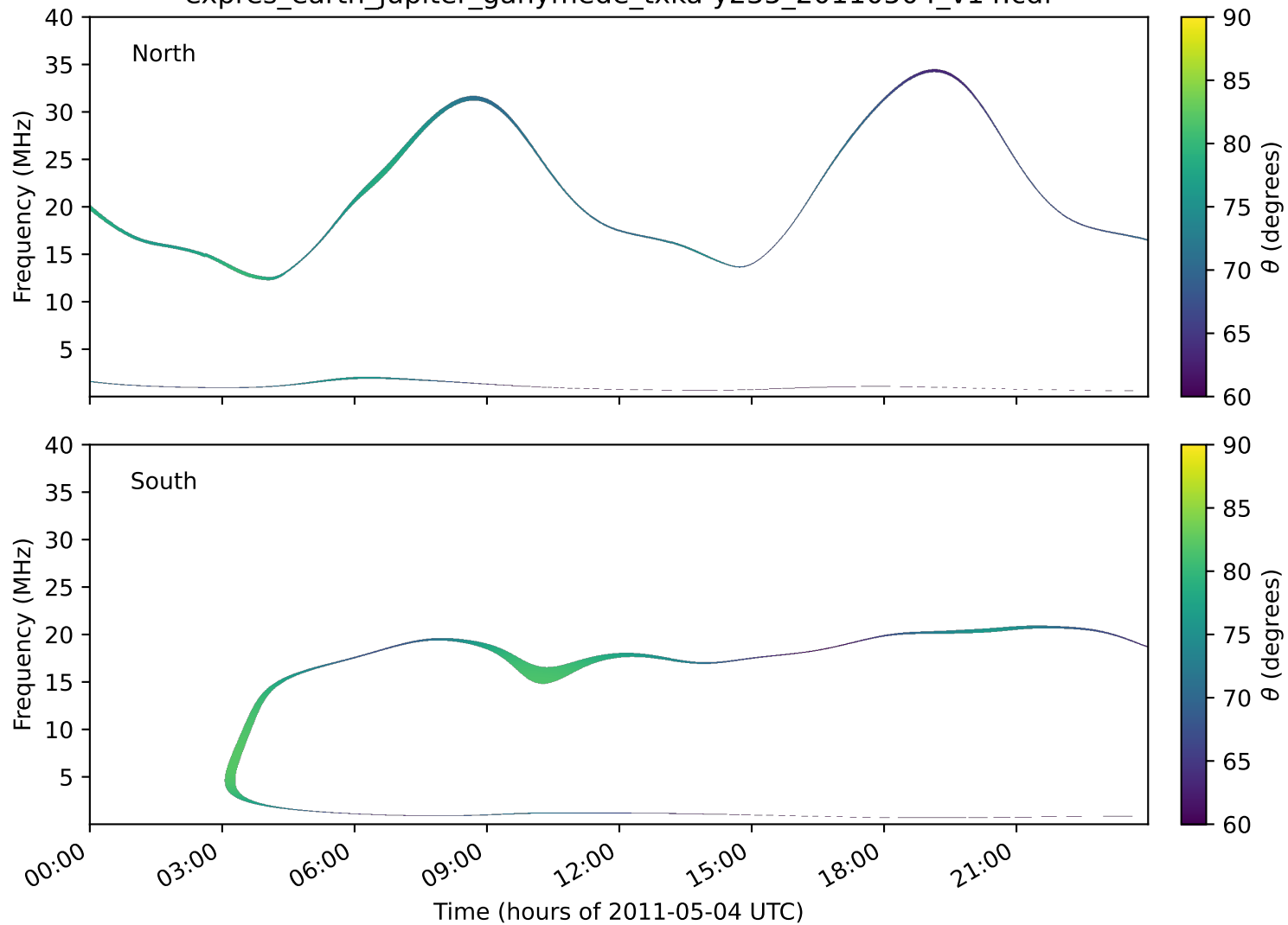
expres_earth_jupiter_ganymede_txka-y235_20110504_v14.cdf
