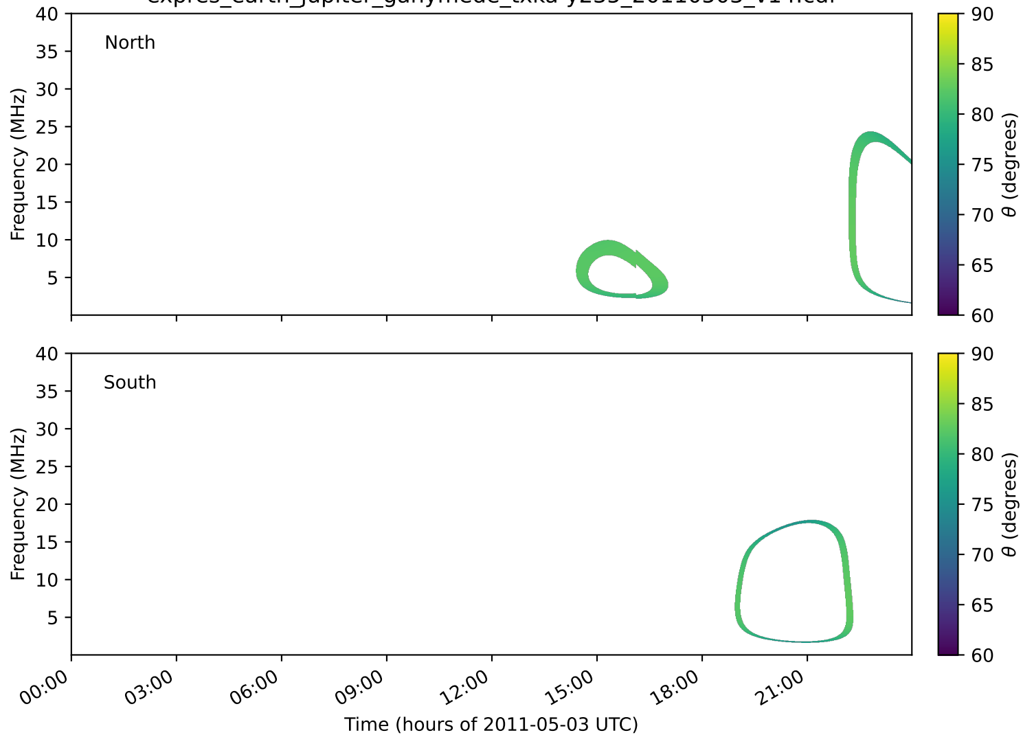
expres_earth_jupiter_ganymede_txka-y235_20110503_v14.cdf
