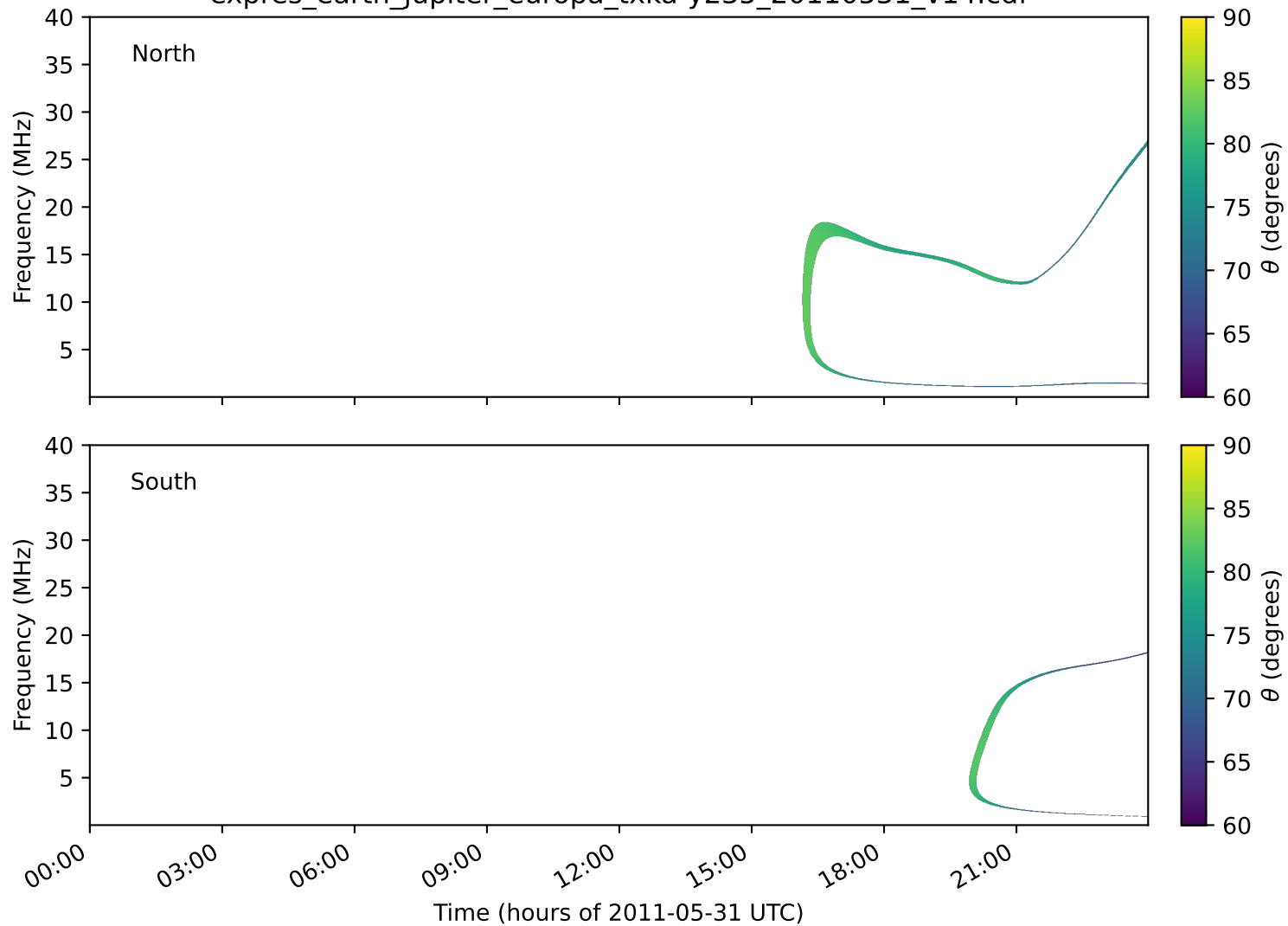
expres_earth_jupiter_europa_txka-y235_20110531_v14.cdf
