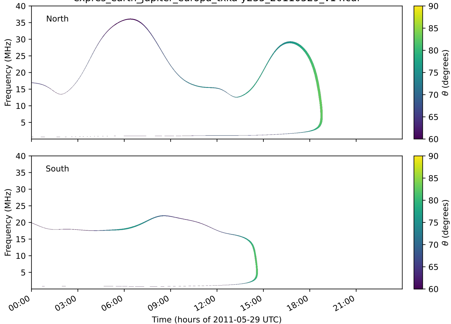
expres_earth_jupiter_europa_txka-y235_20110529_v14.cdf
