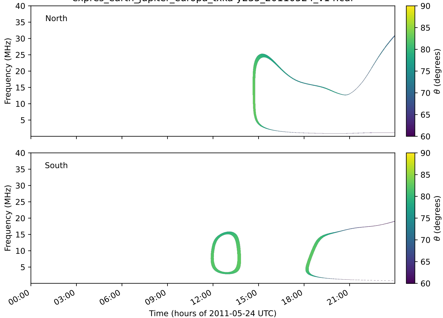
expres_earth_jupiter_europa_txka-y235_20110524_v14.cdf
