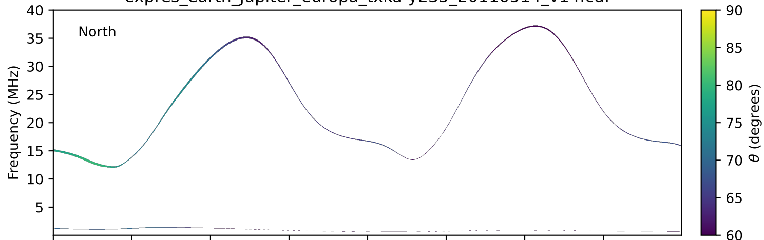
expres_earth_jupiter_europa_txka-y235_20110514_v14.cdf
