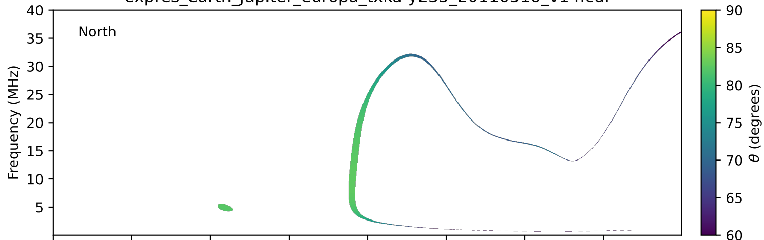
expres_earth_jupiter_europa_txka-y235_20110510_v14.cdf
